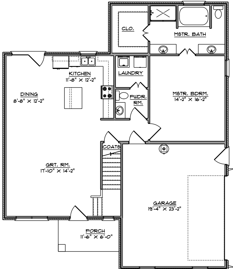
FIRST FLOOR PLAN SCALE: NONE
